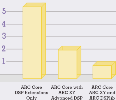
Normalized Performance for 256 point FFT (Number of CPU cycles)
